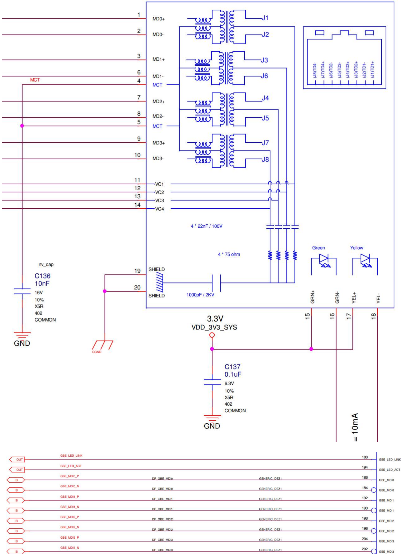
J15 A70-112-331N126 RJ45_POE COMMON
