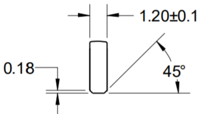
CHAMFEREDGE DETAL
